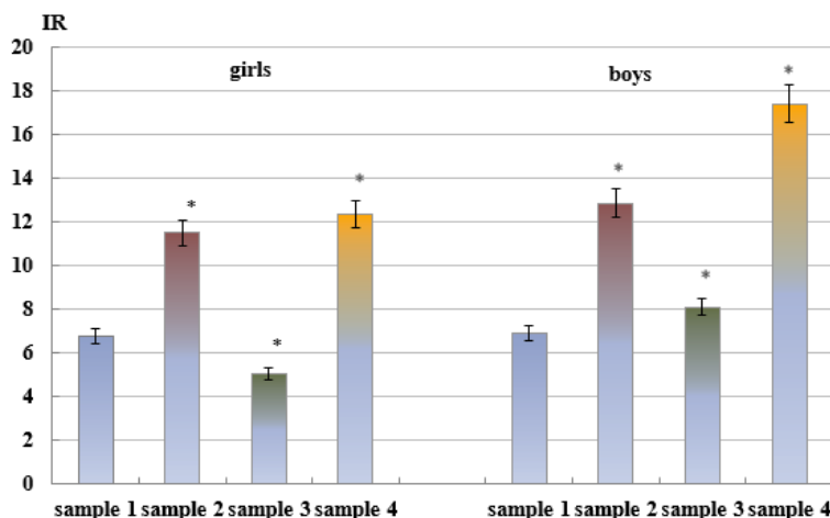
Figure 6. Dynamics of the Ruffier Index (IR) during the educational year
